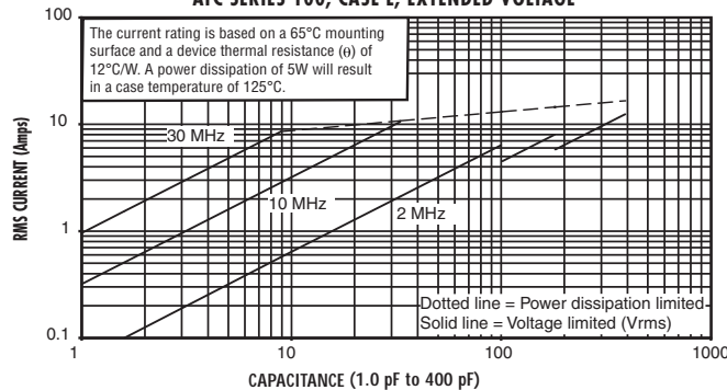
CURRENT RATING VS CAPACITANCE ATC SERIES 100, CASE E, EXTENDED VOLTAGE
