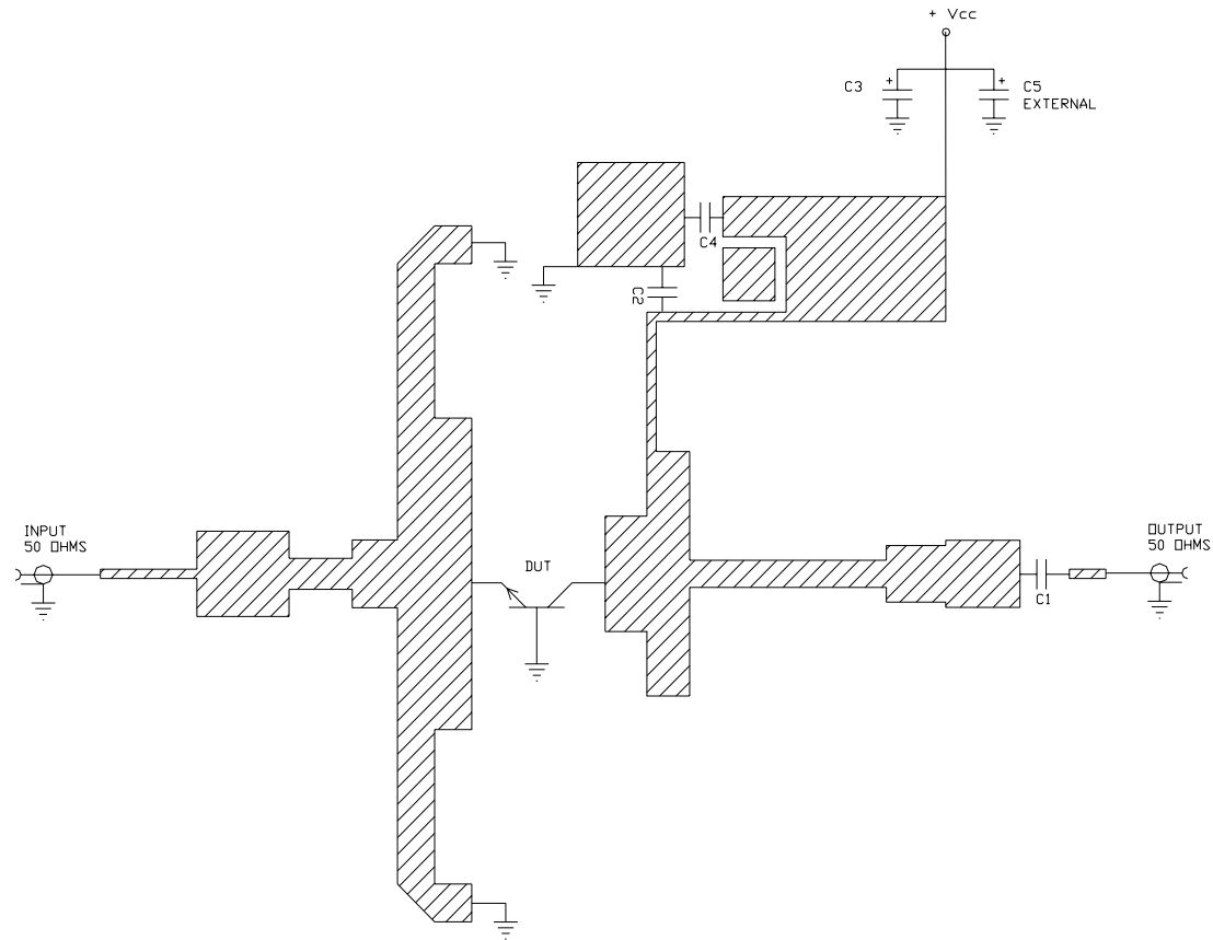
ELECTRICAL SCHEMATIC
