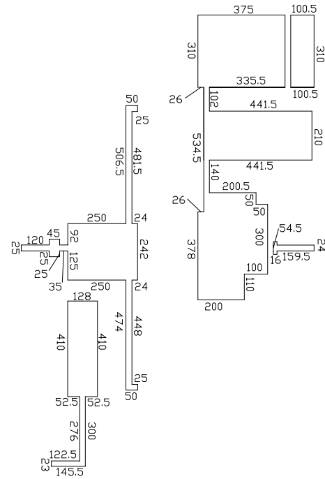
CIRCUIT DIMENSIONS IN MILS
