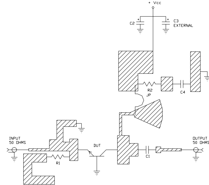
ELECTRICAL SCHEMATIC
